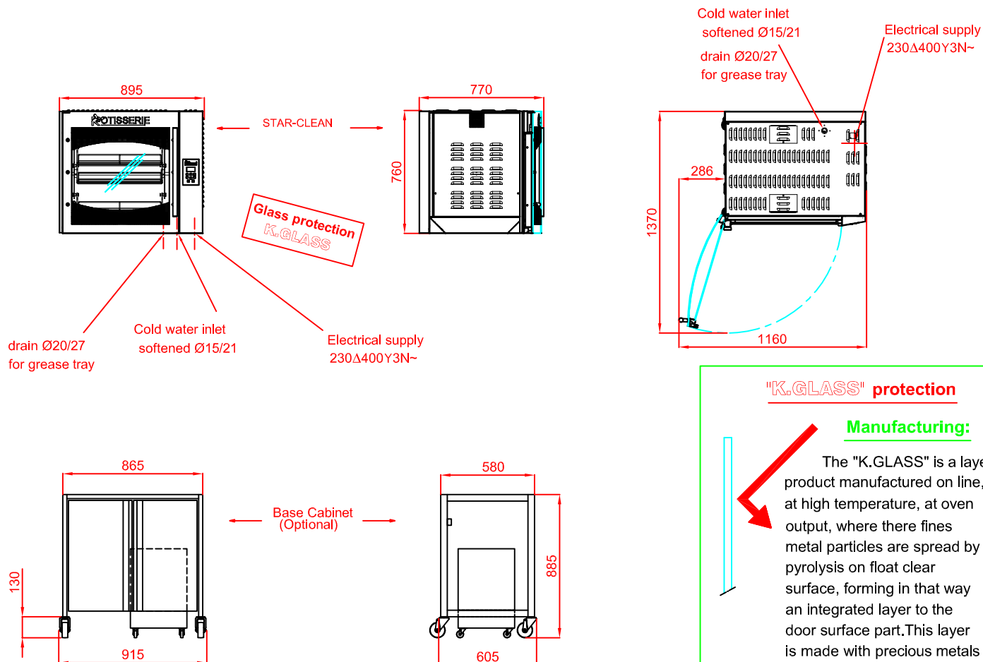
FRONT VIEW
