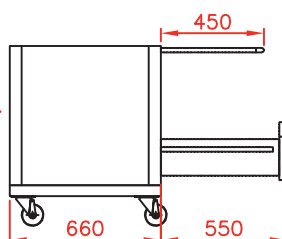
Heated base cabinet with drawers (Optional)
