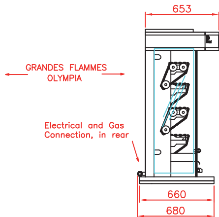
Side view Rotisserie with roof and base on casters (optional)
