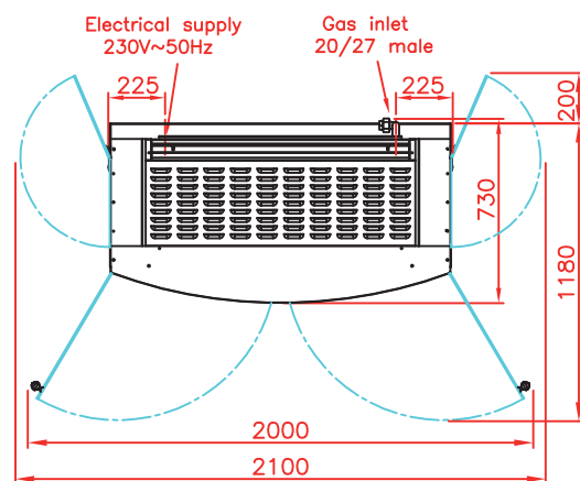
Top view Rotisserie with roof and base on casters (optional)
