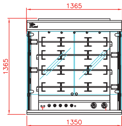
Front view Rotisserie with roof and base on casters (optional)
