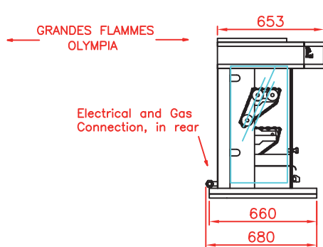
Side view Rotisserie with roof and base on casters (optional)
