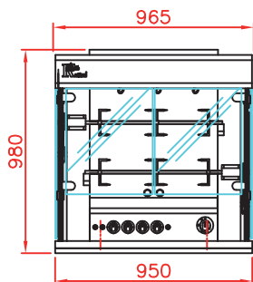
Front view Rotisserie with roof and base on casters (optional)
