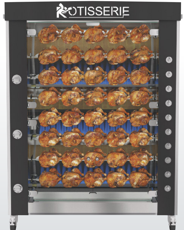
GF1375-8G-SSP Stainless steel with porcelain enamel
