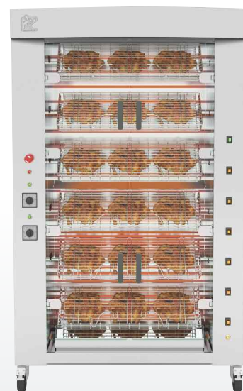
1160.6PAiE Finition inox
