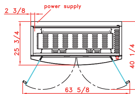
Top view Rotisserie with roof
