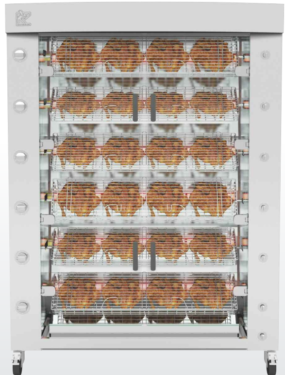
FBS1400-6G-SS Stainless steel and chrome
