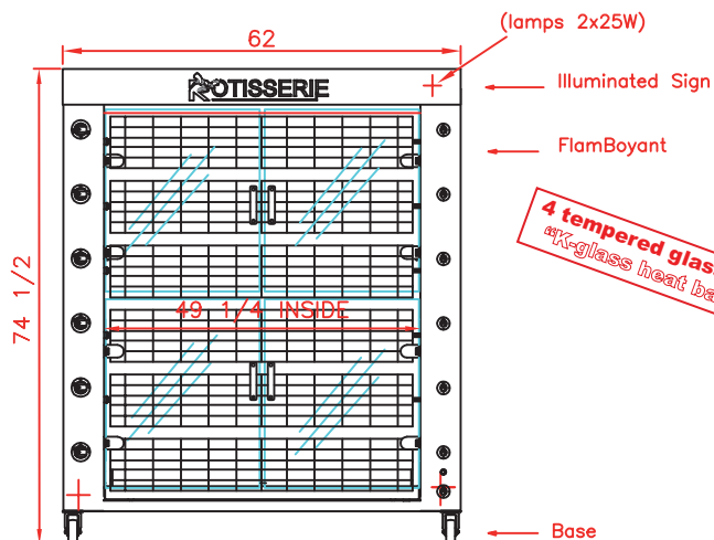
Front view Rotisserie with roof
