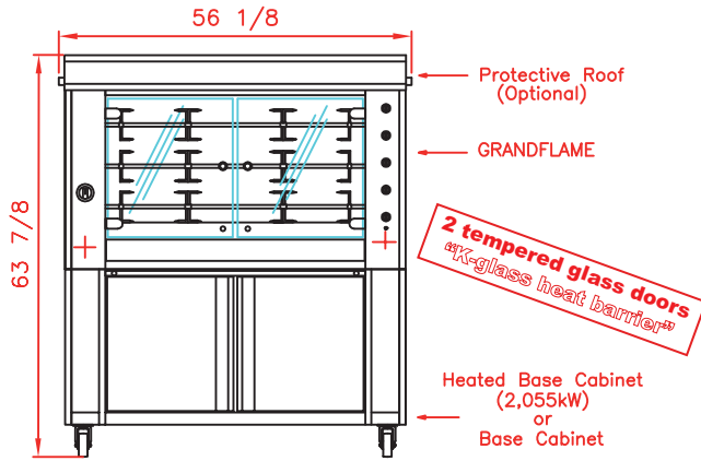
Front view Rotisserie with roof
