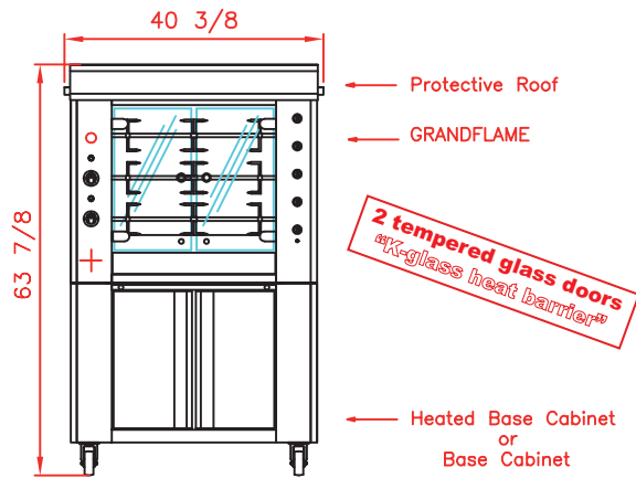
Front view Rotisserie with roof
