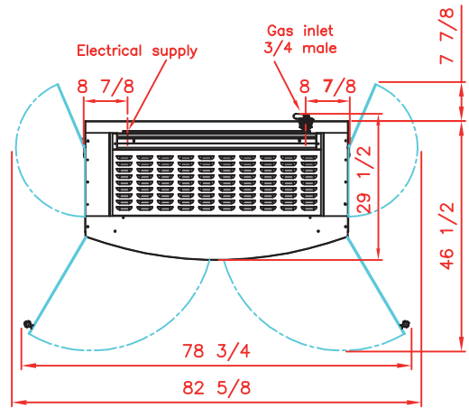
Top view Rotisserie with roof
