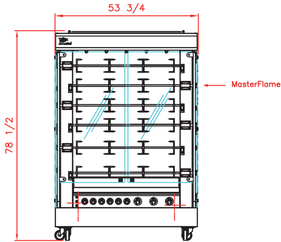
Front view Rotisserie with roof
