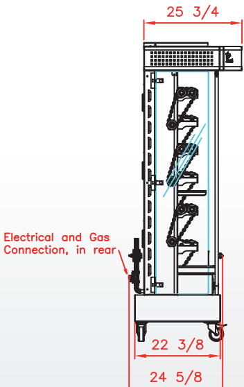
Side view Rotisserie with roof
