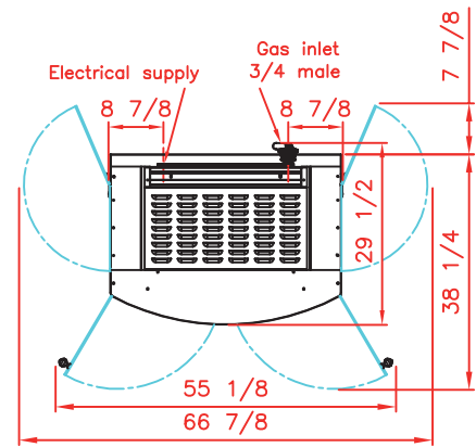
Top view Rotisserie with roof
